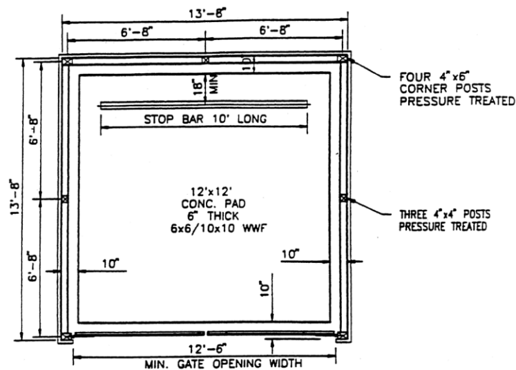
FIGURE XIV-3 DIMENSIONAL REQUIREMENTS AND SPECIFICATIONS FOR TRASH RECEPTACLES
